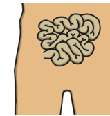
small intestine
