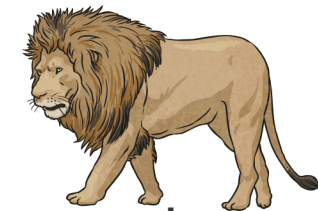
predators
