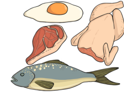
protein
