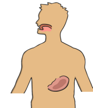
stomach
