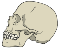
skull
